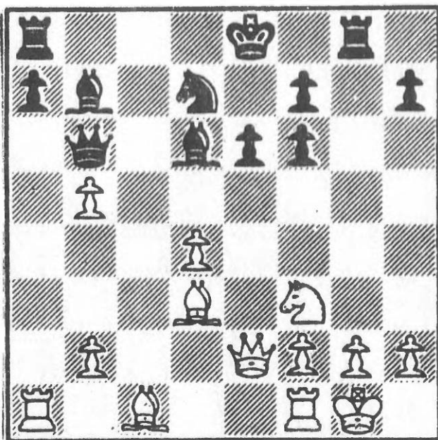
393 After 16 b5
